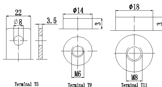
Terminal Dimensions
